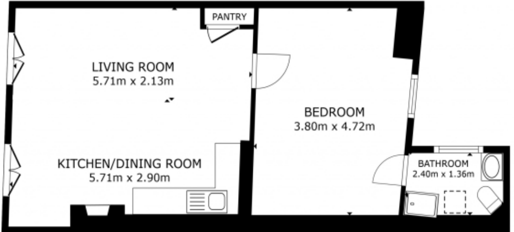
FLOOR PLAN
